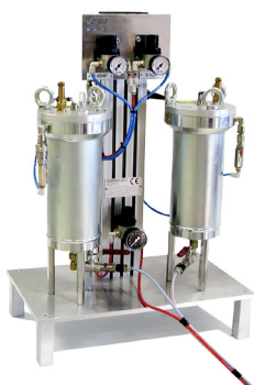
5 litre Feeding tanks
