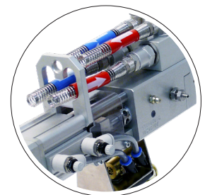
Material recirculation
